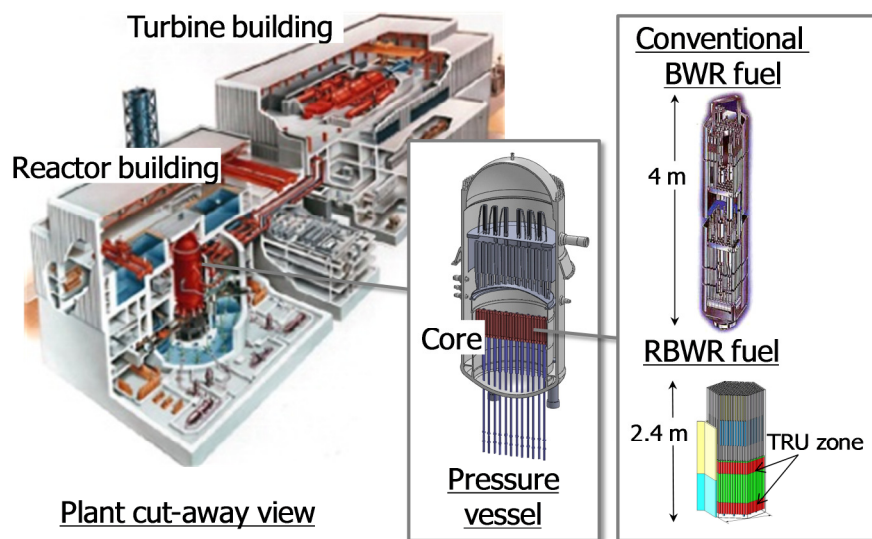
Fig. Outline of RBWR
