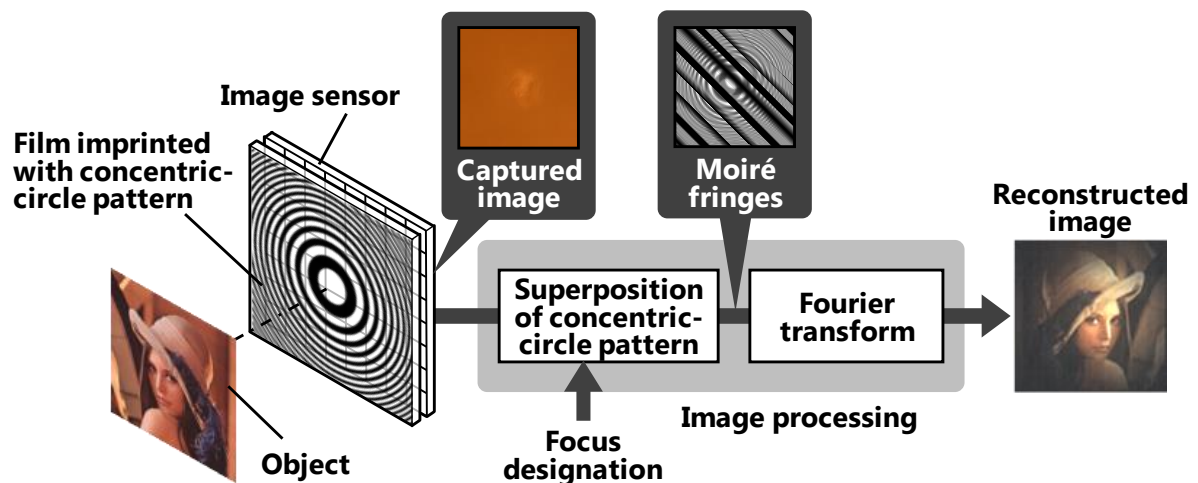
Figure: Principle of newly developed lensless camera technology
